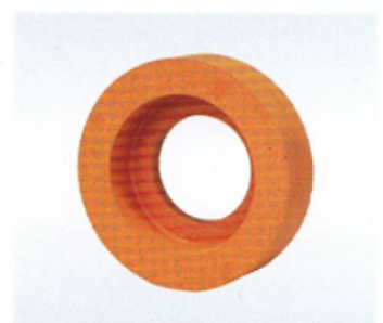
Z016 10S水松抛光轮 10S polish wheel 规格/SIZE : 150×70×40(mm) 150×70×30(mm) 130×60×35(mm) 目数/MESH : 10S40, 10S60, 10S80
