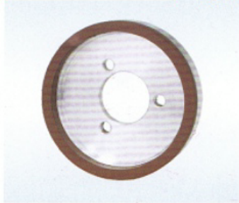
Z009 直边机树脂轮(B型) 颜色(红/绿) Edging machine resin wheel (TypeB)Color (red/green) 规格/SIZE : 150×10×10(mm) 孔径/HOLE : 12mm, 22mm, 50mm 目数/MESH : 180#, 240#, 320#
